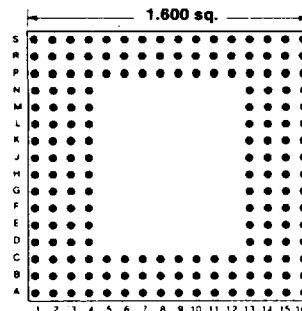
176 PINS Footprint 16007
