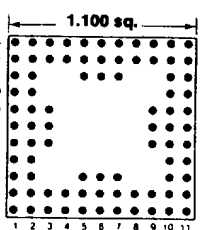
Footprint 11009
