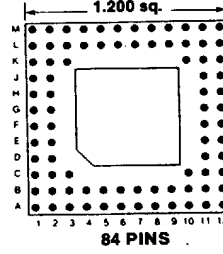
Footprint 12012
