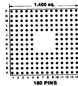
Footprint 14003
