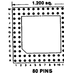
Footprint 12014
