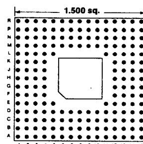
180 PINS Footprint 15009
