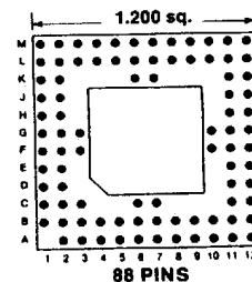
Footprint 12008
