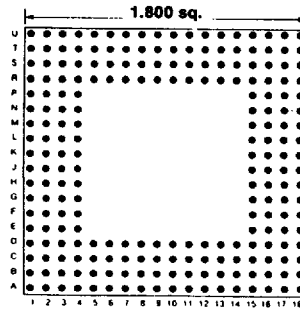
224 PINS Footprint 18005
