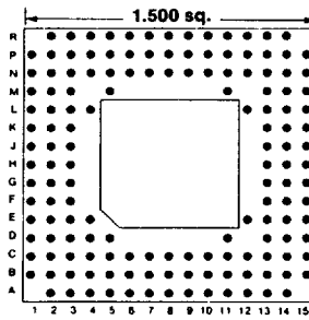
149 PINS Footprint 15018
