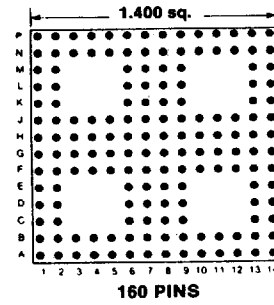
Footprint 14009
