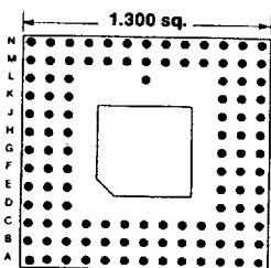
114 PINS Footprint 13051
