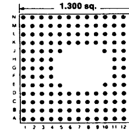
Footprint 13044
