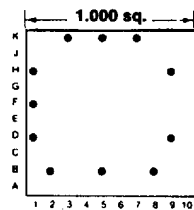
Footprint 10011
