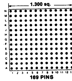
Footprint 13001
