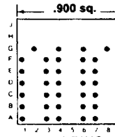
40 PINS Footprint 09015
