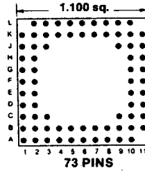
Footprint 11022
