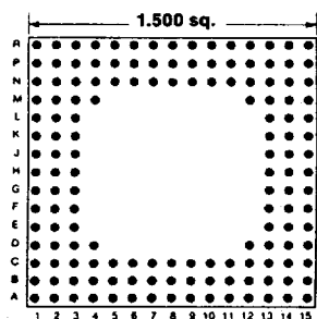
148 PINS Footprint 15022
