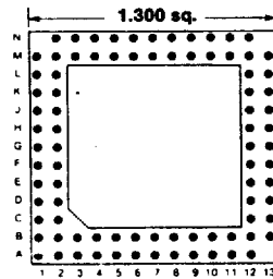
Footprint 13030
