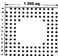
121 PINS Footprint 13058
