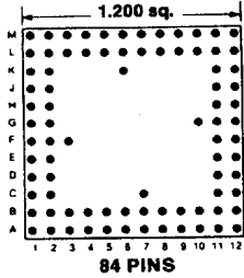
Footprint 12011
