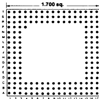
169 PINS Footprint 17002
