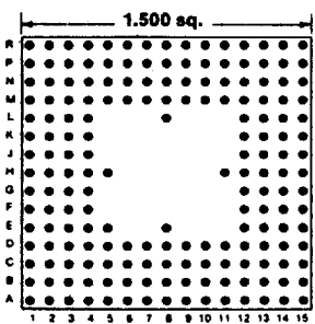
181 PINS Footprint 15006
