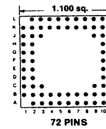
Footprint 11025
