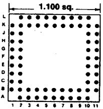
68 PINS Footprint 11033
