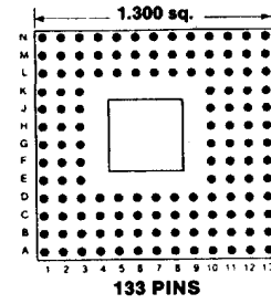
Footprint 13004
