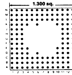
Footprint 13039
