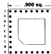
32 PINS Footprint 09016
