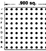
81 PINS Footprint 09001
