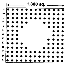
133 PINS Footprint 13052
