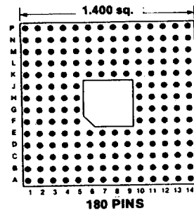
Footprint 14002
