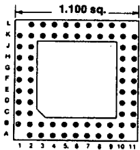
68 PINS Footprint 11032
