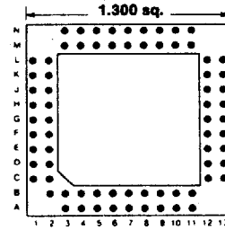
Footprint 13034
