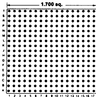
289 PINS Footprint 17001
