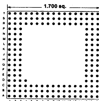
169 PINS Footprint 17012
