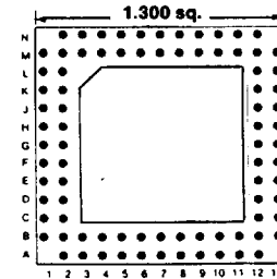
Footprint 13042
