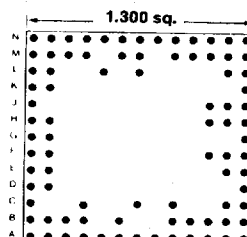
88 PINS Footprint 13057
