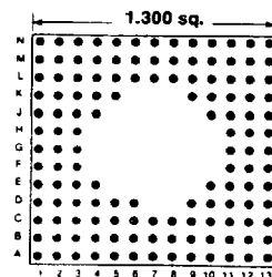
133 PINS Footprint 13055
