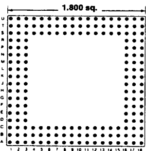
180 PINS Footprint 18007
