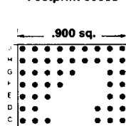
65 PINS Footprint 09006
