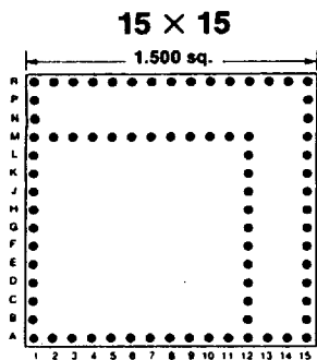
77 PINS Footprint 15037
