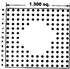
133 PINS Footprint 13054
