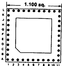
40 PINS Footprint 11043
