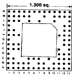
93 PINS Footprint 13045
