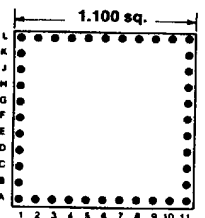
40 PINS Footprint 11044
