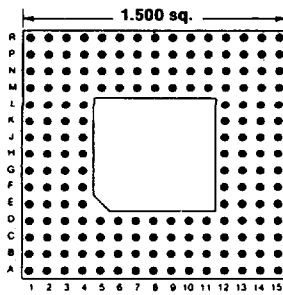
176 PINS Footprint 15013
