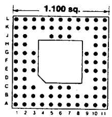
Footprint 11007
