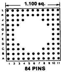
Footprint 11012
