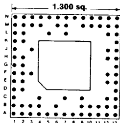
88 PINS Footprint 13049
