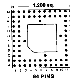
Footprint 12010
