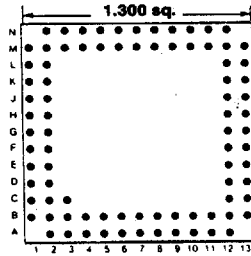
Footprint 13033
