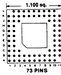
Footprint 11021
