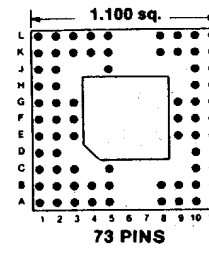
Footprint 11019
