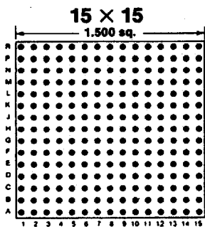
225 PINS Footprint 15001
