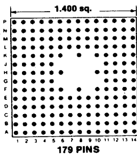
Footprint 14005
