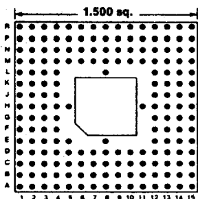
181 PINS Footprint 15005
