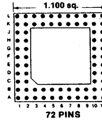
Footprint 11023
