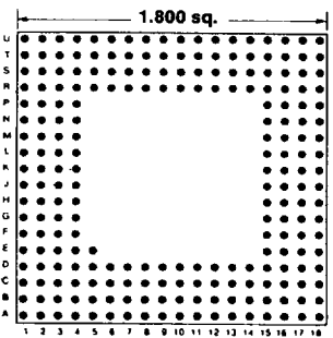
225 PINS Footprint 18003
