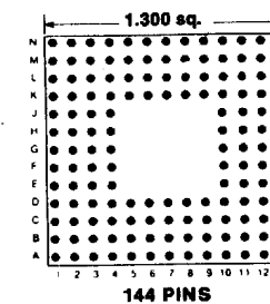
Footprint 13003
