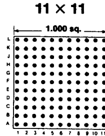
Footprint 11001
