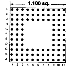
Footprint 11006
