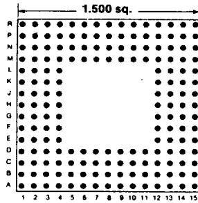
176 PINS Footprint 15014
