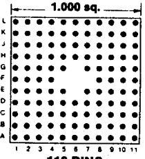
Footprint 11003
