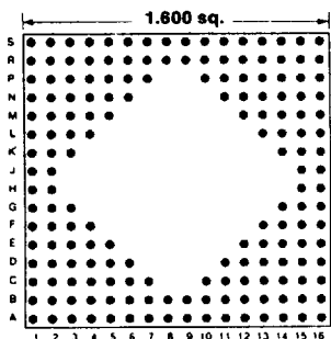
172 PINS Footprint 16002
