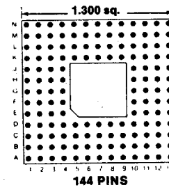
Footprint 13002
