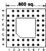
44 PINS Footprint 08002
