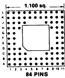
Footprint 11011
