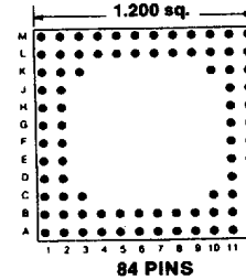
Footprint 12013
