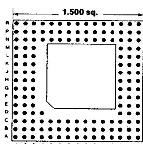
145 PINS Footprint 15023
