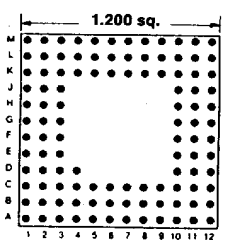
109 PINS Footprint 12003
