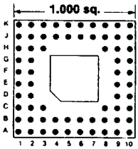
Footprint 10005
