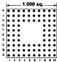
Footprint 10003
