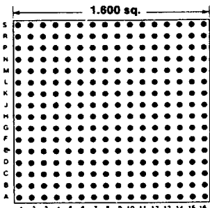
256 PINS Footprint 16001
