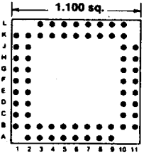
65 PINS Footprint 11037
