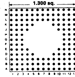
Footprint 13038
