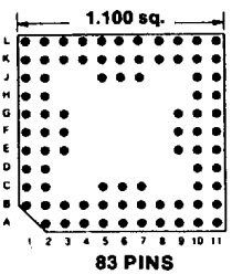
Footprint 11014
