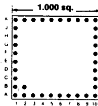
Footprint 10011
