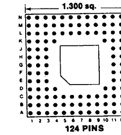
Footprint 13008
