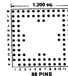
Footprint 12009
