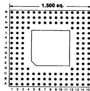
148 PINS Footprint 15021
