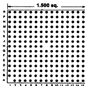
223 PINS Footprint 15003
