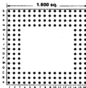
166 PINS Footprint 16004
