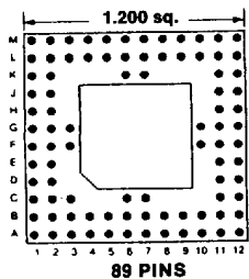
Footprint 12006
