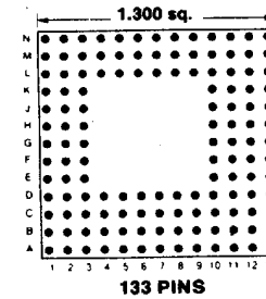
Footprint 13005
