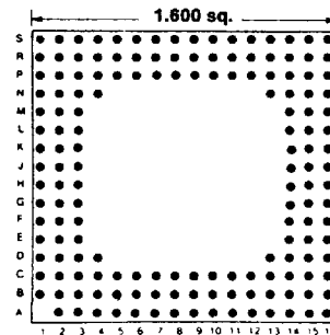
159 PINS Footprint 16009
