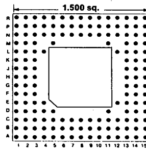
153 PINS Footprint 15016
