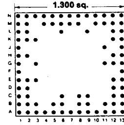
Footprint 13041
