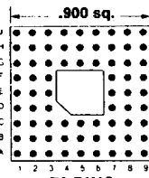
72 PINS Footprint 09003
