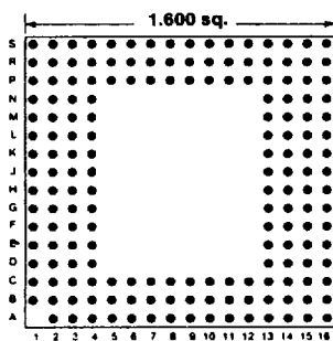
175 PINS Footprint 16010
