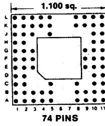
Footprint 11017
