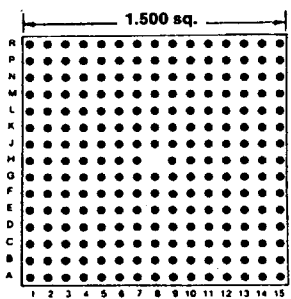
224 PINS Footprint 15038
