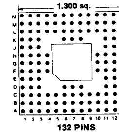
Footprint 13006
