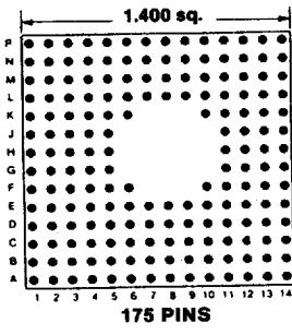
Footprint 14006
