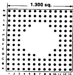
133 PINS Footprint 13046
