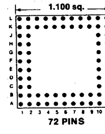
Footprint 11024
