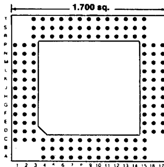
144 PINS Footprint 17005
