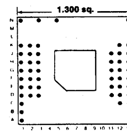
Footprint 13036
