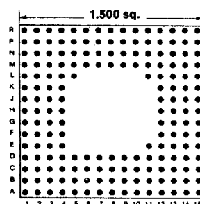
179 PINS Footprint 15012
