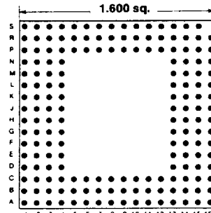
175 PINS Footprint 16008
