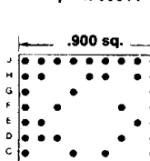
49 PINS Footprint 09012
