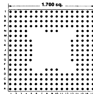
225 PINS Footprint 17008
