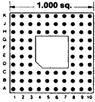
Footprint 10002
