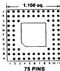
Footprint 11015
