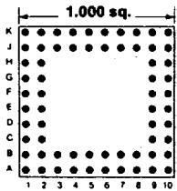
Footprint 10010
