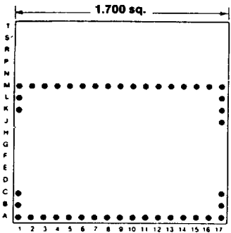
43 PINS Footprint 17014
