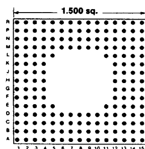
180 PINS Footprint 15010
