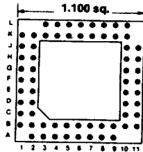
65 PINS Footprint 11036
