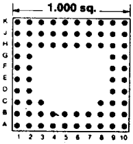
Footprint 10004
