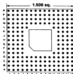
179 PINS Footprint 15011
