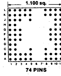
Footprint 11018
