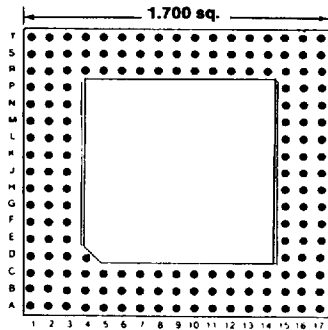
169 PINS Footprint 17013
