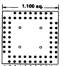
65 PINS Footprint 11038
