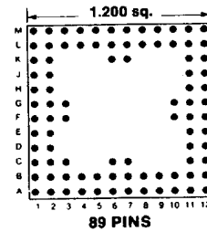
Footprint 12007
