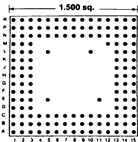
149 PINS Footprint 15020
