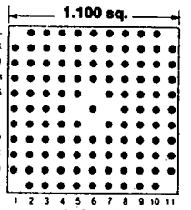
Footprint 11004
