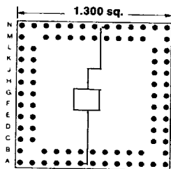
84 PINS Footprint 13056
