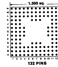
Footprint 13007
