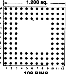
108 PINS Footprint 12005
