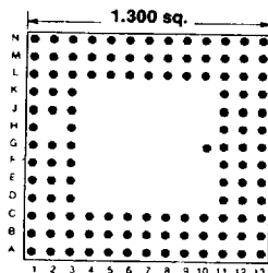
113 PINS Footprint 13050
