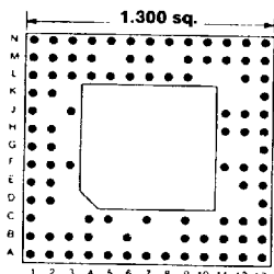
95 PINS Footprint 13047
