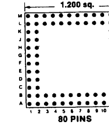
Footprint 12015
