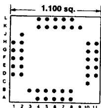
44 PINS Footprint 11042
