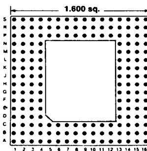
176 PINS Footprint 16006
