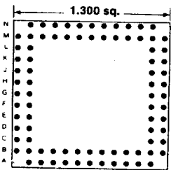
84 PINS Footprint 13053
