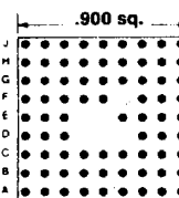
75 PINS Footprint 09002
