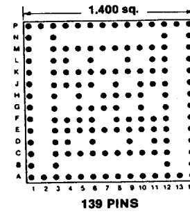
Footprint 14010
