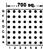
49 PINS Footprint 07001
