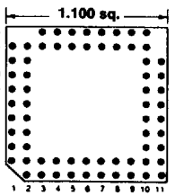
67 PINS Footprint 11035
