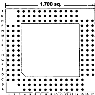
145 PINS Footprint 17003
