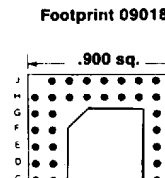
52 PINS Footprint 09019
