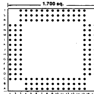
144 PINS Footprint 17006
