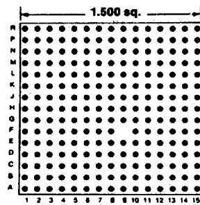
224 PINS Footprint 15002
