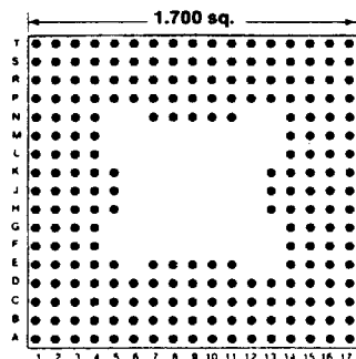
225 PINS Footprint 17007
