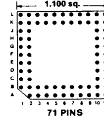
Footprint 11027
