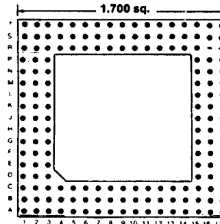
168 PINS Footprint 17009
