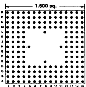
180 PINS Footprint 15008
