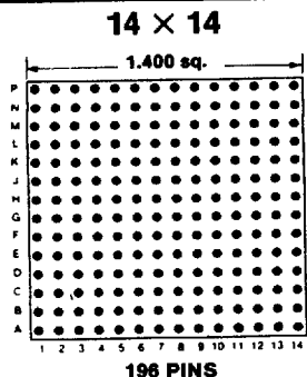
Footprint 14001
