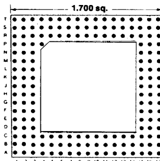
169 PINS Footprint 17010
