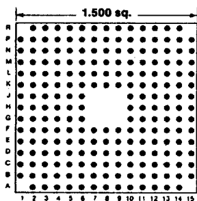
212 PINS Footprint 15004
