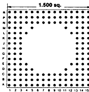
153 PINS Footprint 15017
