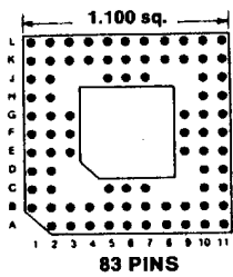
Footprint 11013
