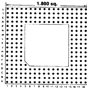
225 PINS Footprint 18002
