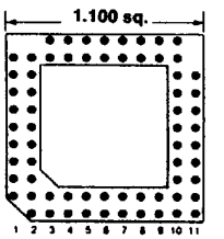
67 PINS Footprint 11034
