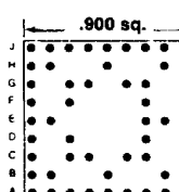
53 PINS Footprint 09011
