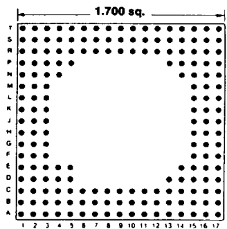
181 PINS Footprint 17015
