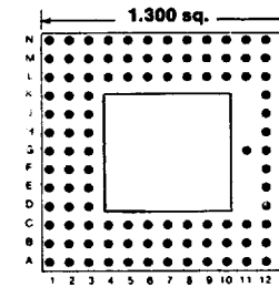
Footprint 13040
