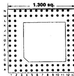
Footprint 13032
