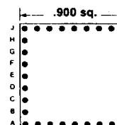
32 PINS Footprint 09017
