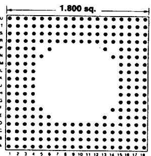
233 PINS Footprint 18008
