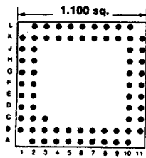
69 PINS Footprint 11031
