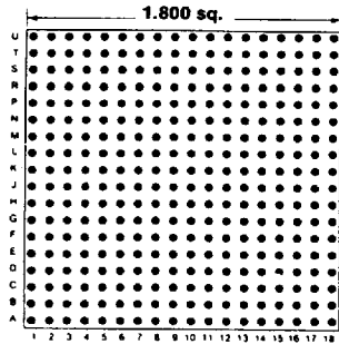
324 PINS Footprint 18001
