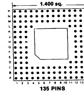
Footprint 14011
