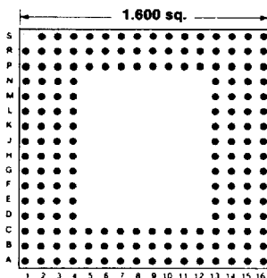
175 PINS Footprint 16003
