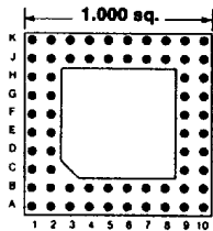
Footprint 10009
