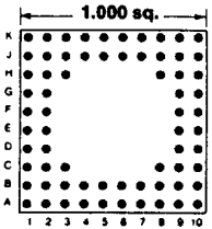
Footprint 10005
