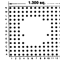
Footprint 13043
