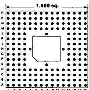
180 PINS Footprint 15007
