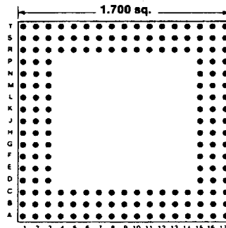
168 PINS Footprint 17011
