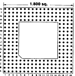
224 PINS Footprint 18004
