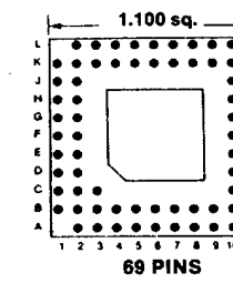
Footprint 11030
