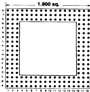
180 PINS Footprint 18006
