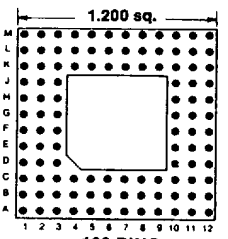
108 PINS Footprint 12004
