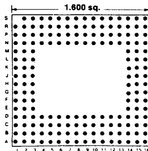
175 PINS Footprint 16005
