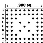
65 PINS Footprint 09005
