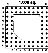
Footprint 10007
