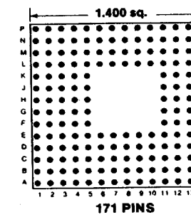
Footprint 14008
