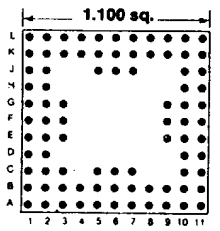
Footprint 11008
