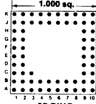
Footprint 10008
