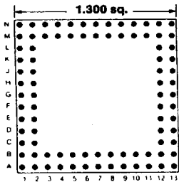
Footprint 13029
