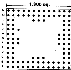
100 PINS Footprint 13059
